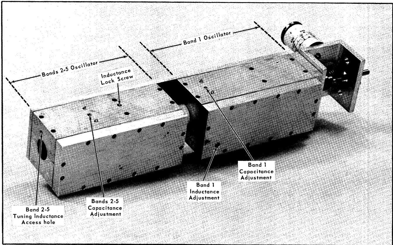
Fig. 6-29. Local Oscillator adjustments.
