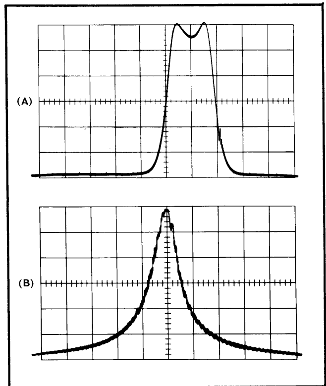
Fig. 6-11. Typical spectrum display for final Resolution adjustments (Step 4).
