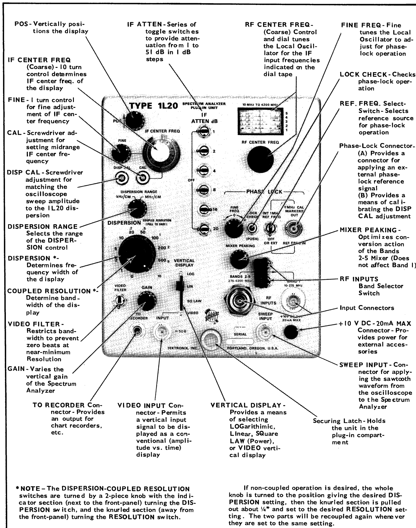
Fig. 2-1. Function of Type 1L20 front-panel controls and connectors.
