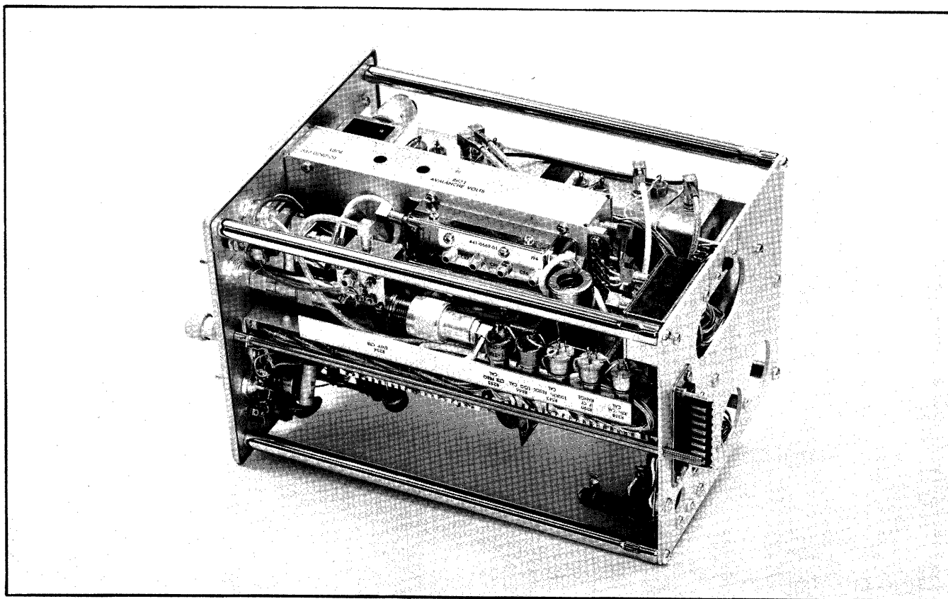
Fig. 4-3. Wiring and cable connections to Phase-Lock assembly.
