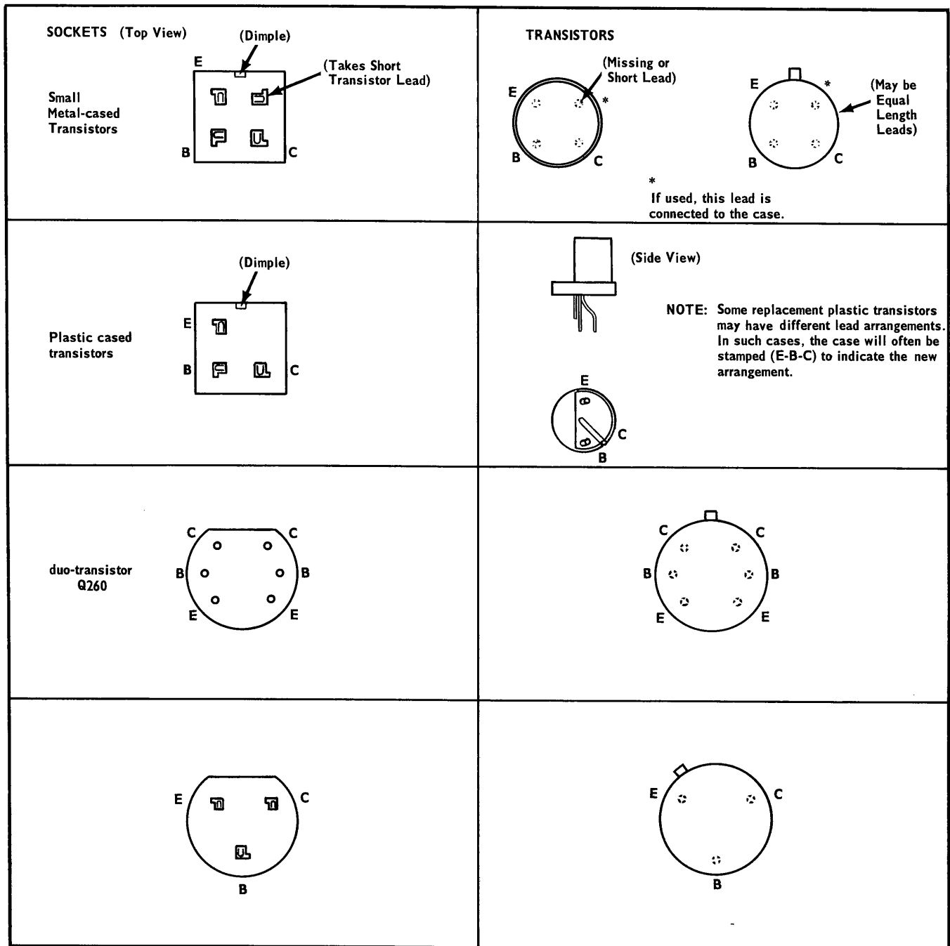
Fig. 4-5. Transistor lead and socket connections as viewed from the top of the chassis.
