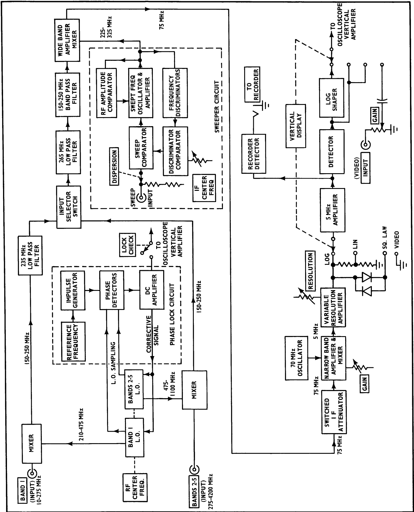
Fig. 3-1. Block Diagram of the Type 1L20.
