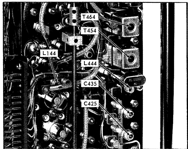
Fig. 6-16. Location of IF Amplifier adjustments (Step 9).
