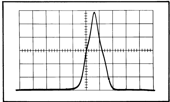
Fig. 6-10. Typical spectrum display for adjusting R543 (Step 4).
